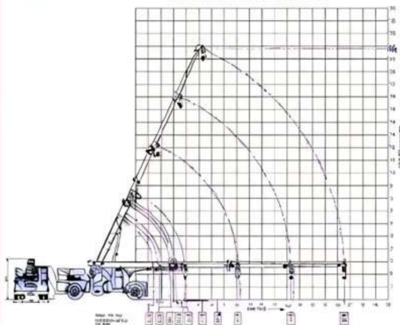
LOAD CHART SNF 20
